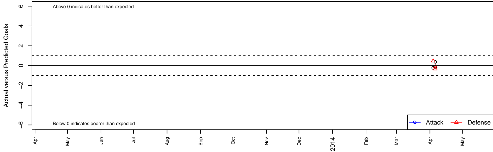
Seattle Celtic White B99 Dots are actual minus expected GF (blue circles) and GA (red triangles). Blue line is smoothed change in attack strength. Red is smoothed change in defense strength.
